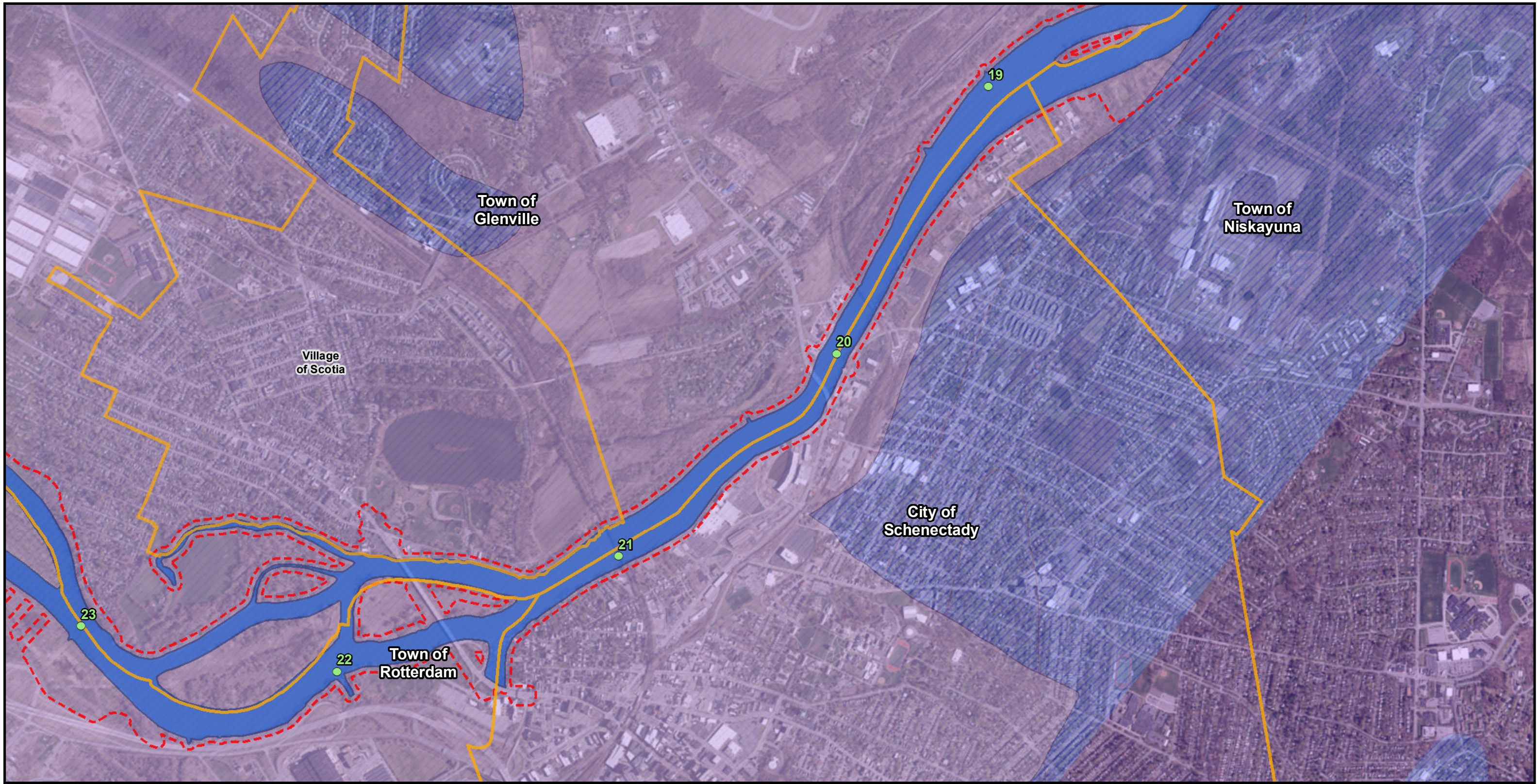
Figure 23F: Aquifers
